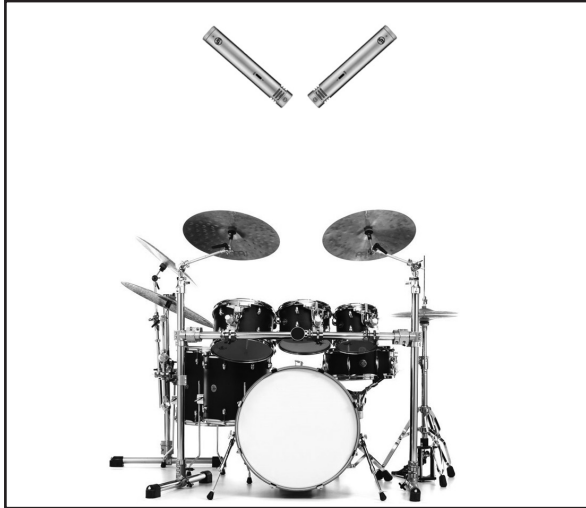
In this diagram, two WA-84's are used in a coincident pair, also known as XY configuration, to record stereo drum overheads.
