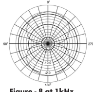
Figure - 8 at 1kHz
