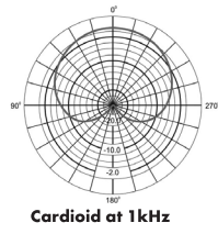
Cardioid at 1kHz
