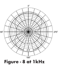
Figure - 8 at 1kHz
