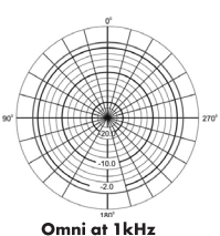
Omni at 1kHz
